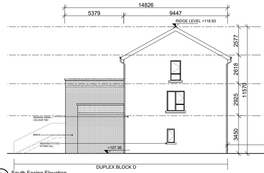
3 South Facing Elevation 0461
